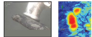
SBI UXO Survey Results: Verification of Magnetometer Targets
